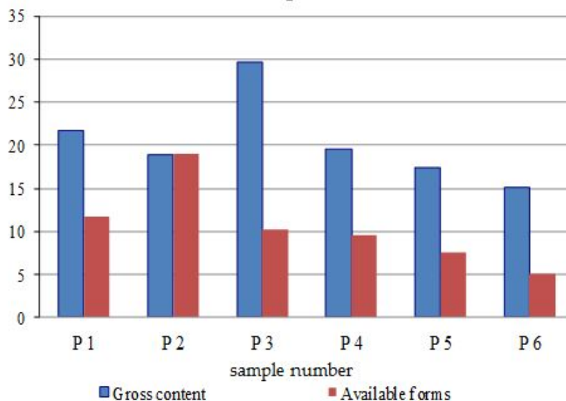
Figure 2. Lead content in soils, mg/kg.
